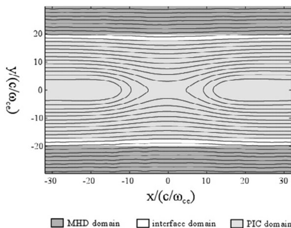
Fig. 2: Magnetic field lines of force in multi-hierarchy simulation.
