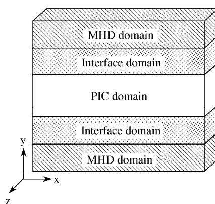
Fig. 1: Schematic diagram of the multi-hierarchy simulation model.
