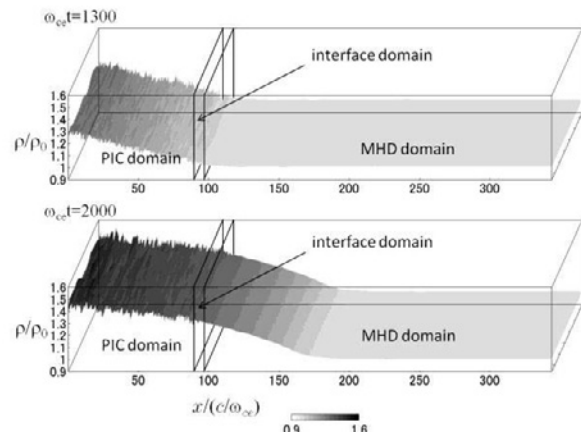
Fig. 1: Bird's eye view of the spatial profile of plasma mass density at \omega_{ce}t=1300 and at \omega_{ce}t=2000 . Plasmas smoothly propagate from the PIC to MHD domains.
