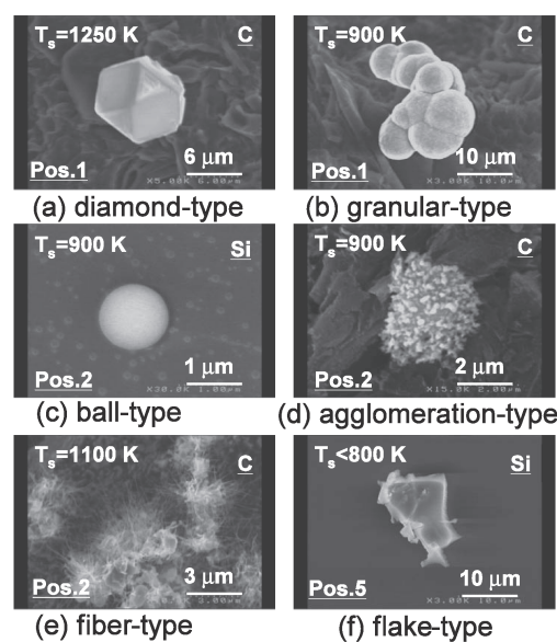
Fig. 2 SEM pictures of carbon dust on the graphite targets and silicon crystal targets.
