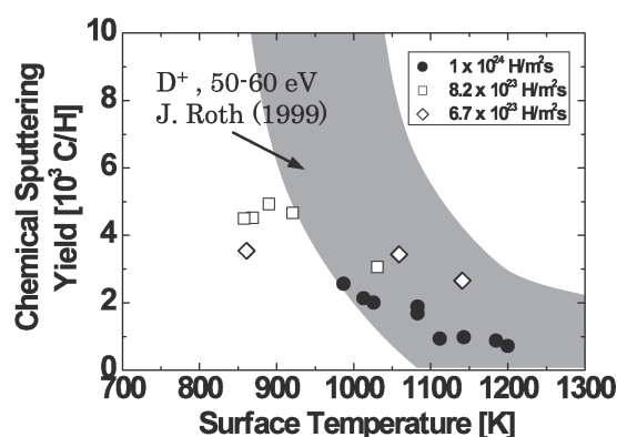
Fig. 1 Temperature dependence of chemical sputtering yield estimated by the weight loss of graphite targets.
