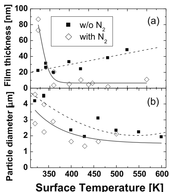
Fig. 1. Surface temperature dependence of film thickness (a) and diameter of single carbon dust particles (b) observed on the target exposed to H 2 /CH 4 and H 2 /CH 4 /N 2 plasmas for 10 hours. The gas flow rate of H 2 , CH 4 , and N 2 were 20, 1 and 1 sccm, respectively.
