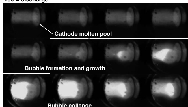
Fig. 1 Frame by frame pictures of abrupt cathode material ejection the from the molten cathode pool after bubble formation and growth. Frame rate is 23000 fps.
