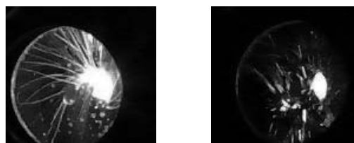
Fig. 2 Fine droplets ejection from the molten cathode pool just after arc termination. Exposre time is 1/8,000 s(left) and 1/10,000 s(right).
