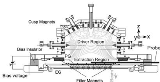
Fig. 1. Extraction and driver regions in the R&D ion source in NIFS NBI teststand. Connection of the bias power supply is shown on the left hand side.
