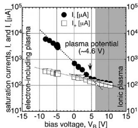
Fig. 2. Negative and positive saturation currents (closed circles and open squares, respectively) with respect to bias voltage.
