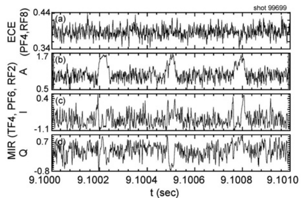
Fig. 2 ECE and MIR signal in the case of EHO.
