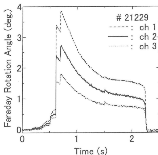
Fig. 3 The measured Faraday rotation angle of a pellet injected plasma.
