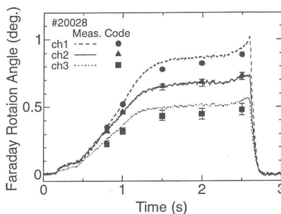
Fig. 2 Comparison of the time evolution of the Faraday rotation angle with calculation from interferometer data.
