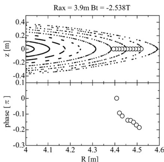
Fig.2 The view points on Poincaré map of magnetic field line and the phase of heat pulse fluctuation measured by RADM.
