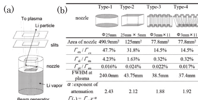
Fig. 1 Results of numerical simulation for various nozzles
