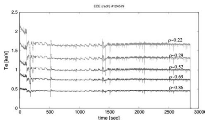
Fig. 1. The evolution of the electron temperature in the longest discharge of 2013 campaign.
