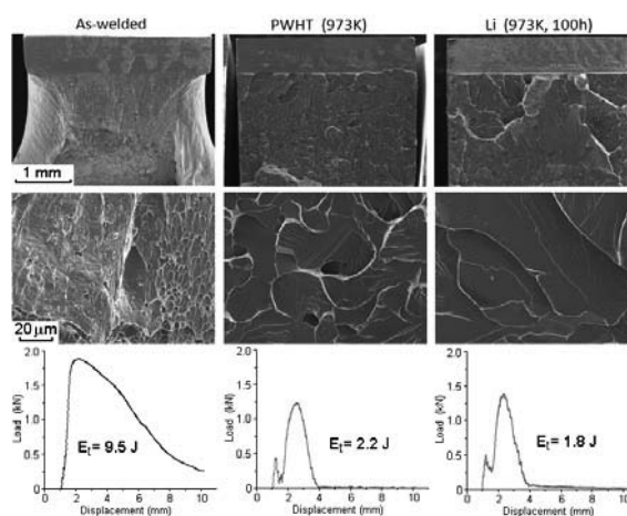
Fig. 2. Fractography and corresponding load-displacement curves of V-4Ti-4Cr alloy obtained after impact test at 77 K depending on pre-treatment: as-welded conditions; after PWHT at 973 K and after exposure to Li at 973 K.
