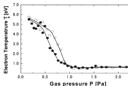
Fig. 2 Dependence of hydrogen gas pressure P on the electron temperature T_e at a discharge current of 50A. The geometry of the target plates are the oblique target ( \circ ) and the V-shaped target ( \bullet ).
