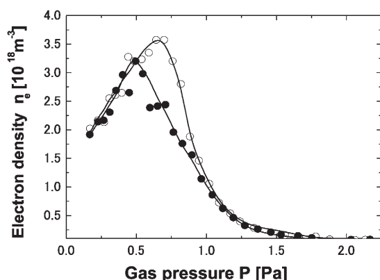
Fig. 1 Dependence of hydrogen gas pressure P on the electron density n_e at a discharge current of 50A. The geometry of the target plates are the oblique target ( \circ ) and the V-shaped target ( \bullet ).
