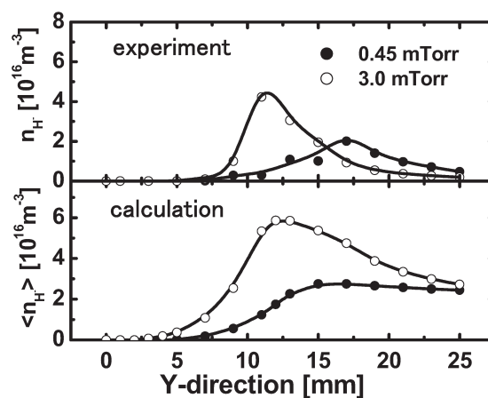
Fig.1 Spatial distributions of measured n_{H^-} and calculated number of hydrogen negative ions \langle n_{H^-} \rangle at gas pressures of 0.45 and 3.0 mTorr.
