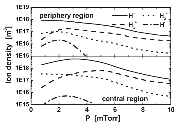
Fig.1 Characteristics of the calculated ion densities ( H^+ , H_2^+ , H_3^+ and H^- ) in the periphery region and central region are plotted against gas pressure P .
