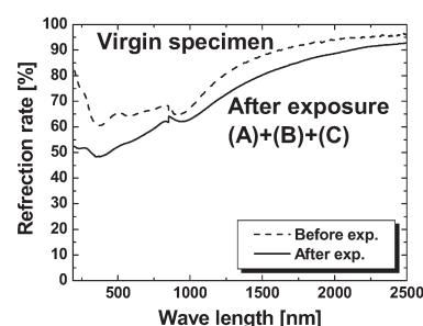
Fig. 2. Optical reflectivity of Mo ((A)+(B)+(C) in table 1) before and after exposure to helium discharges.
