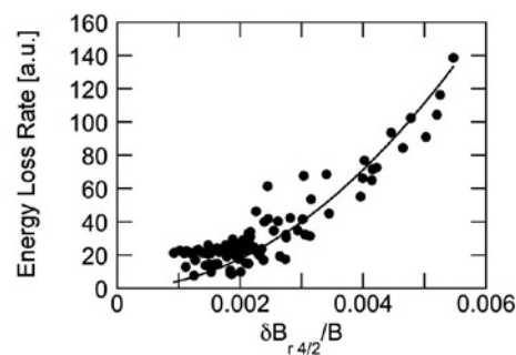
Fig. 2. Stored beam energy loss rate vs. radial magnetic fluctuation amplitude with m/n=4/2 at 10 \leq t \leq 20 ms for nonlinear MHD run with \nu = \nu_n = \eta / \mu_0 = 5 \times 10^{-7} v_A R_0 . Data points are plotted every 0.1 ms. Solid line is a quadratic fit to the data.
