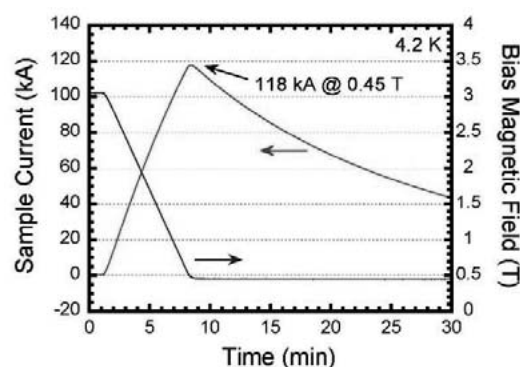
Fig.1 Temporal evaluations of the current of the 100-kA HTS conductor sample and the bias magnetic field of the 9-T split coils.
