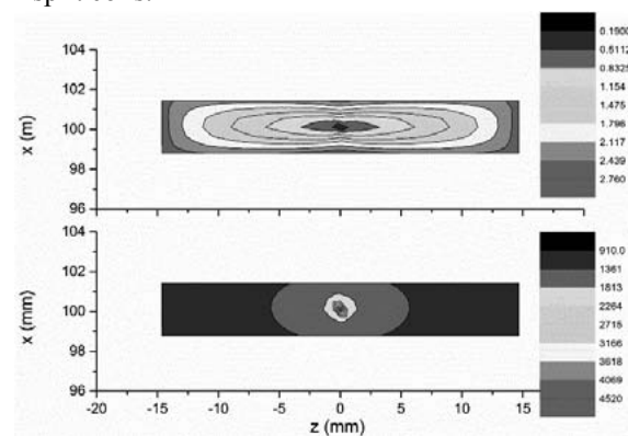
Fig.2 Calculated distributions of the magnetic field and critical current density in the 100-kA conductor sample at 4.2 K, 0.45 T.
