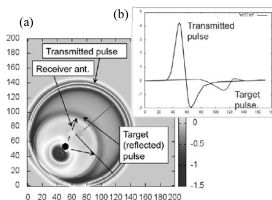
Fig. 2: (a) FDTD simulation of reflecting microwave pulse with a 10mm diameter dielectric object. (b) Transmitted and target reflected pulses at the receiver antenna.
