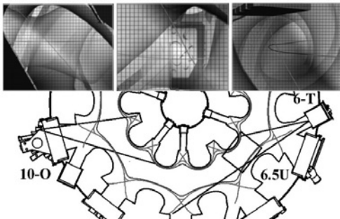
Fig. 1: Fields of view of the IRVB cameras that were installed on three ports of LHD, and CAD images of three cameras with channel numbers.
