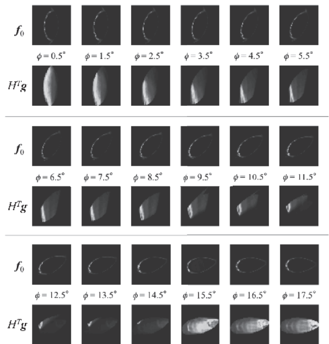
Fig. 2: 3D phantom f_0 calculated by EMC3-EIRENE (upper rows), and 3D back-projection image H^T g (lower rows); both are displayed in poloidal R - Z planes with 32 \times 32 pixelation and at every toroidal angle \phi = 1^\circ , sequentially.
