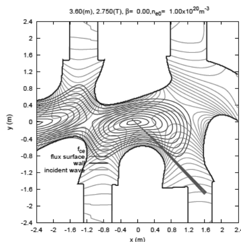
Figure 1: Ray tracing in LHD plasma with density of 10^{20} \text{ m}^{-3} for frequency of 400 GHz.
