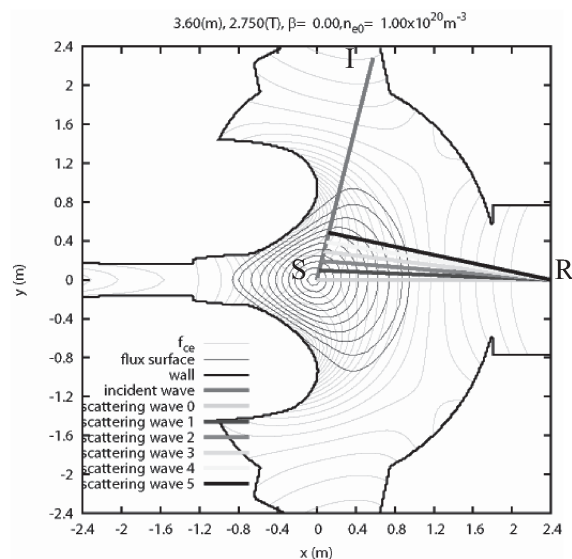
Figure 1: Configuration of injection and scattering beams chosen for feasibility study of LHD-CTS.
