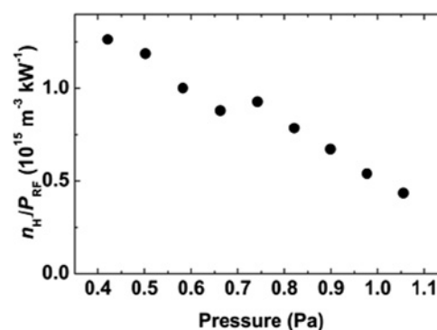
Fig. 2. Source pressure dependence of the H^- density normalized by RF power. The H^- density increased as the pressure decreased.
