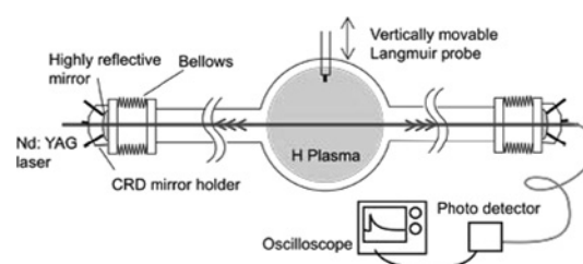
Fig. 1. Cross sectional view of the CRD system installed near the plasma grid in the FET-based ion source. The cavity length was \sim 1.3 m and the plasma length was \sim 0.1 m. Bellows were attached for mirror angle alignment.
