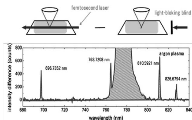
Fig.2 Spectrum increment caused by femtosecond laser pulses. Scattered light from the femtosecond laser is overwritten (760-800 nm)
