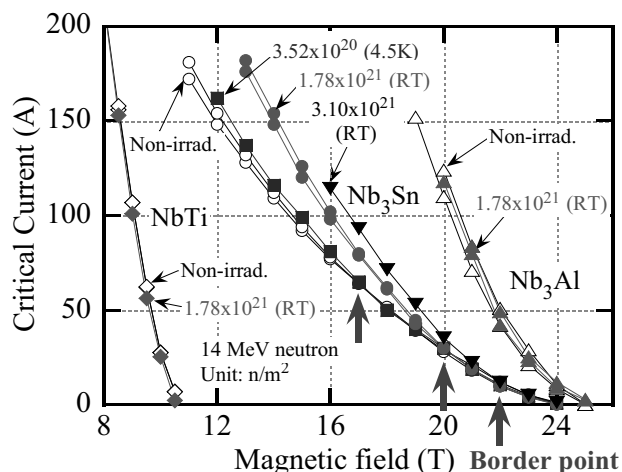
Fig. 1. Change in critical current against magnetic field after 14 MeV neutron irradiation.
