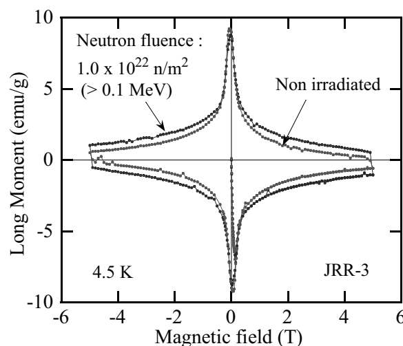
Fig. 3. Results of magnetization measurement comparing non-irradiated sample and irradiated one up to 1.0 \times 10^{22} n/m 2 at JRR-3.
