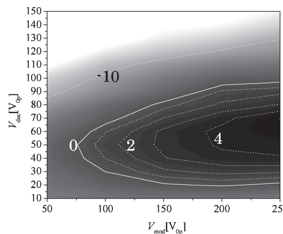
Fig. 3. Calculated Deceleration Efficiency with V_n = -2 kV.
