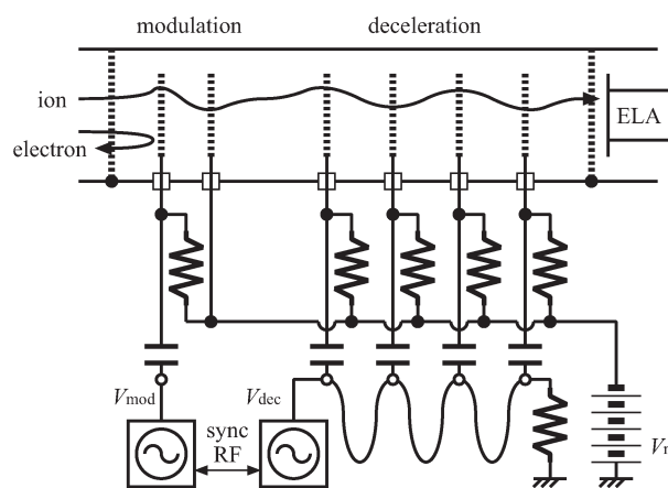
Fig. 1. Schematic diagram of a bias-type TWDEC.
