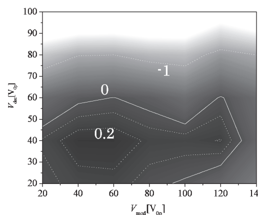
Fig. 2. Calculated Deceleration Efficiency with V_n = 0 .
