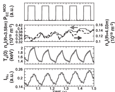
Fig. 2 Wave-forms of modulated ECH power, center and edge line integrated densities, center electron temperature and H\alpha emission intensity.
