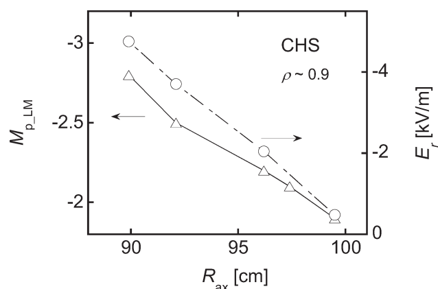
Fig. 2. The dependence of the poloidal Mach number at the transition and the radial electric field formed after the transition on the magnetic axis position in CHS.
