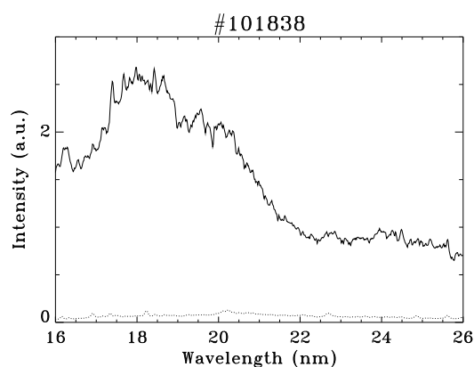
Fig. 1: Spectrum in the 20 nm region measured in the LHD plasma with a tungsten pellet injection.
