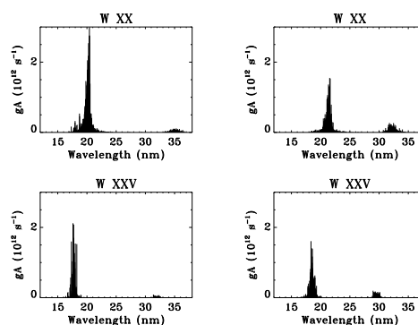
Fig. 2: Calculated distributions of wavelengths and gA values for n = 5-5 transitions of W XX and W XXV. Configurations with even and odd parities are shown separately.
