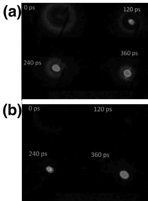
Fig. 1: X-ray framing images. (a) CDBr implosion (b) CD implosion.
