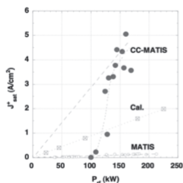
FIG. 2 Rf power dependence of J+sat in CC-MATIS and MATIS, and by calculation using a simple analytical model.
