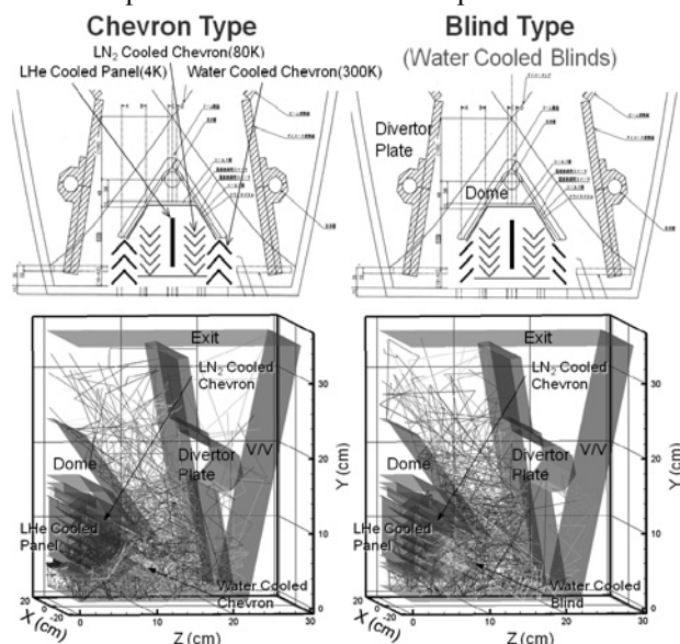
Fig. 1 Models of the components of the CHD and the pumping system for the neutral particle transport simulation (chevron type (left), and blind type (right)).
