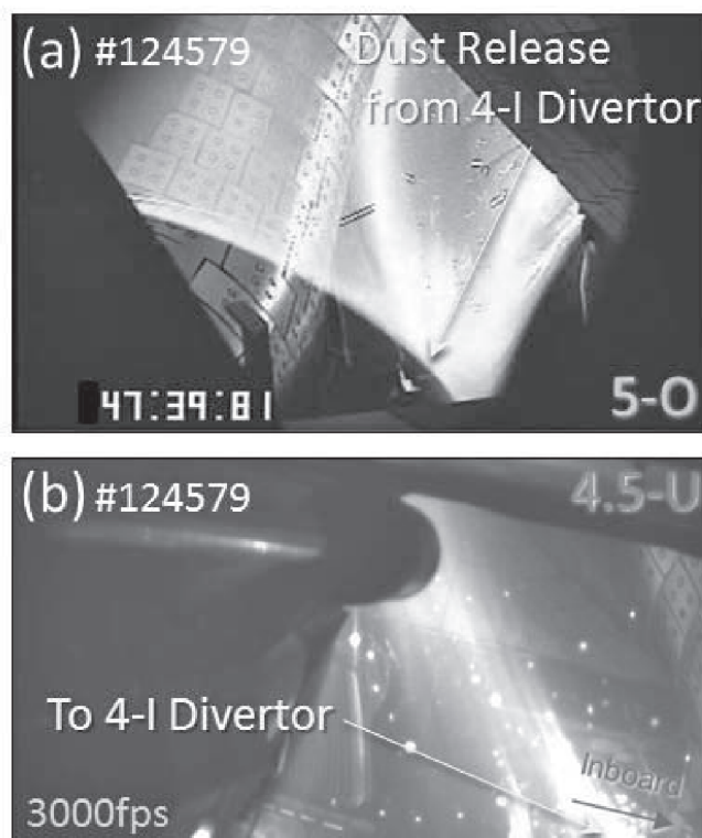
Fig. 1. Image of a LHD plasma viewed from an outer port (5-O) at the end of a long pulse discharge taken with a standard video rate CCD camera (a), an image taken with a fast framing camera installed in an upper port (4.5-U) at the end of the discharge (b).
