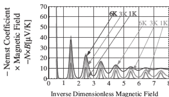
Figure 2: Scaling plots of the Nernst coefficient against 1/B : The curves indicate the results at T=1,3,6 K, respectively. The gray curve corresponds to the ballistic transport.
