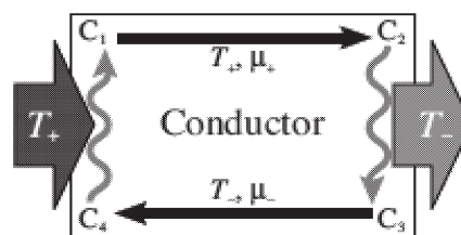
Figure 1: A schematic view of the dynamics of electrons in a Hall bar under the setup for the Nernst effect.
