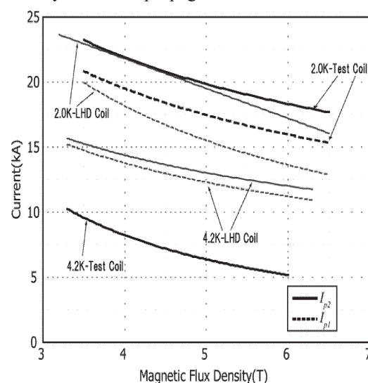
Fig. 2 Stability test results for the test conductor at 4.2K(HeI) and at 2.0K(HeII, 1atm), and test results for the LHD conductor for comparison.
