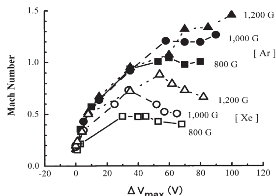
Fig. 2. Dependence of \Delta Mach number on voltage difference for various magnetic fields.
