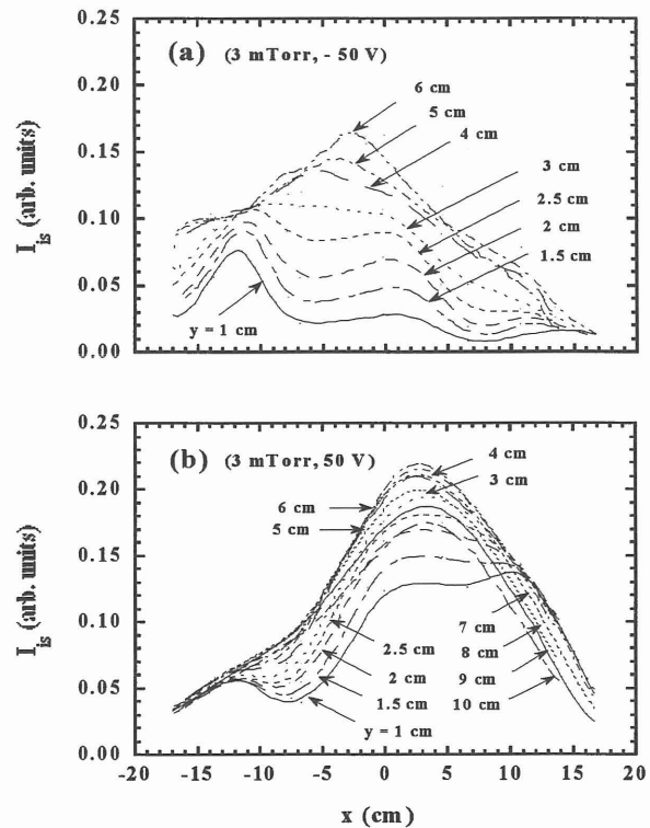
Fig. 2. Radial profiles of ion saturation current ( P = 3 mTorr)
