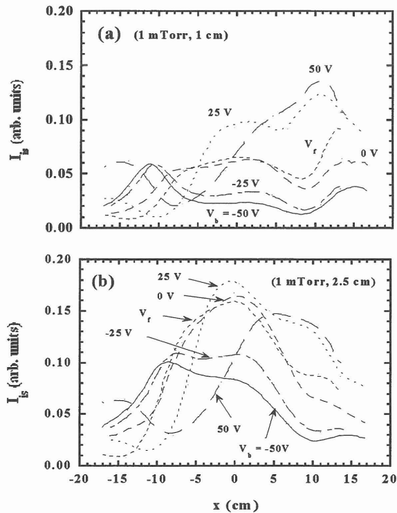
Fig. 1. Radial profiles of ion saturation current ( P = 1 mTorr)
