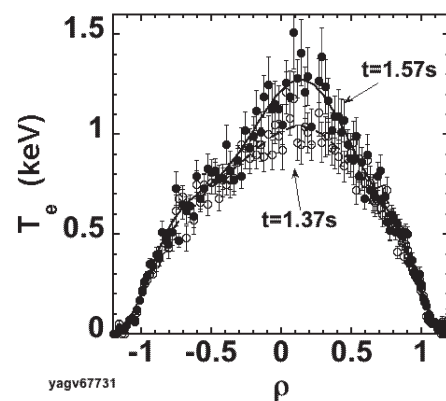
Fig. 2: Electron temperature profiles just before ( t=1.37\text{sec} ) and during ( t=1.57\text{sec} ) ECH. \rho is the normalized minor radius.
