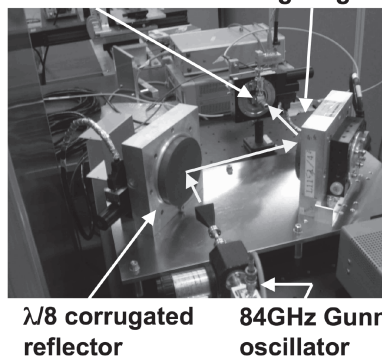
Polarization monitor \lambda/4 corrugated reflector & rotating stage
