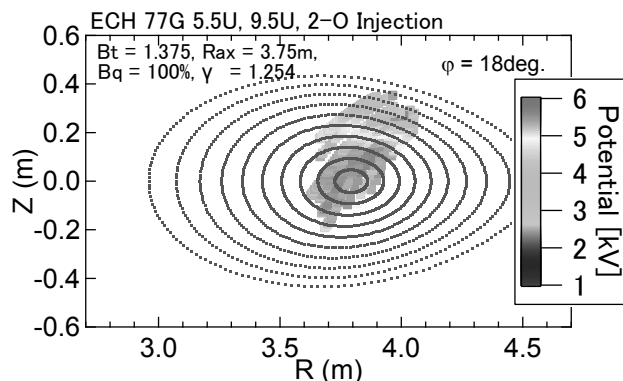
Fig. 2. Obtained 2-D potential profile with HIBP from 7 shots, by changing the probe beam energy
