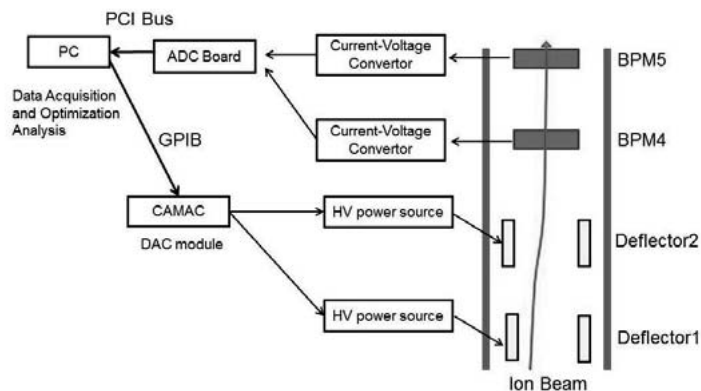
Fig. 1. Simple diagram of automatic beam adjustment system is shown.
