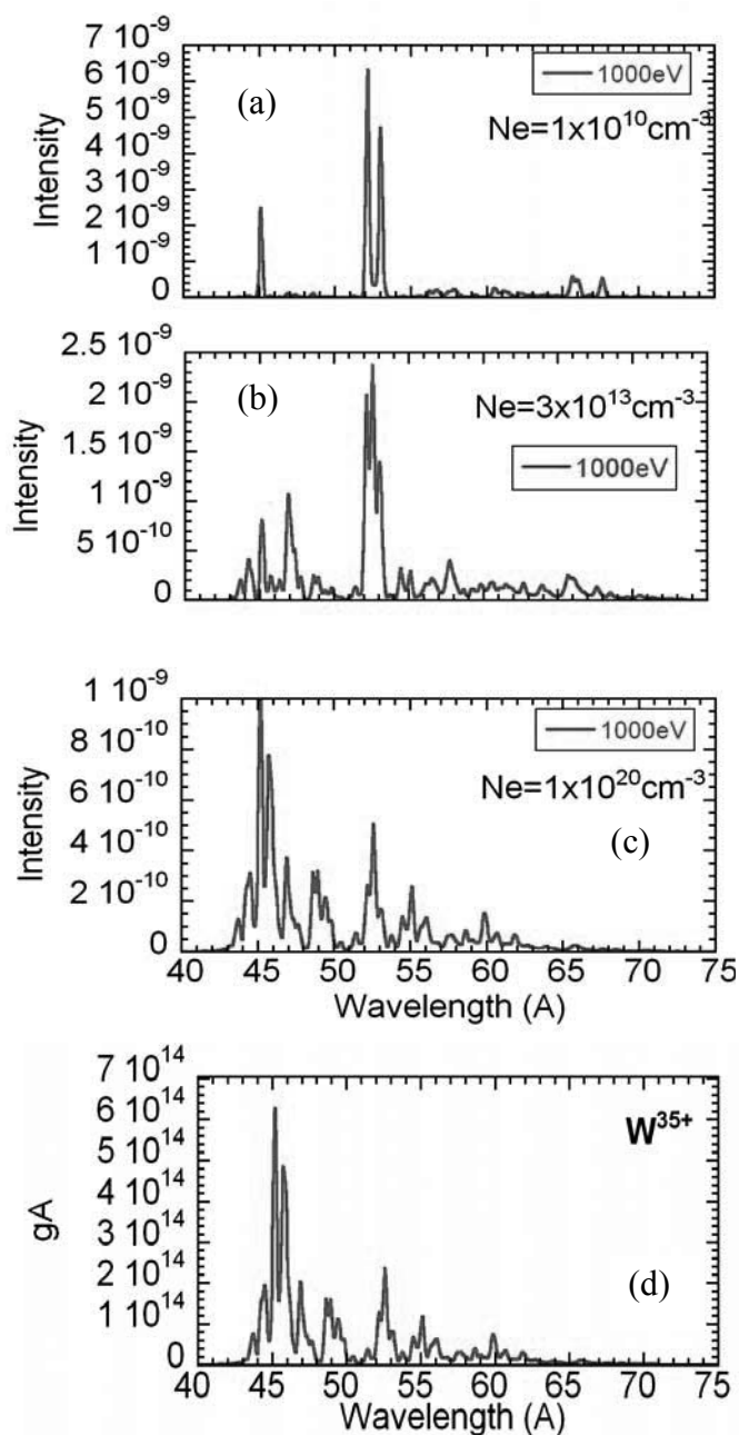
Figure 1. EUV spectra calculated with a collisional-radiative model for W^{35+} with electron temperature 1keV and electron density 10^{10}\text{cm}^{-3} (a), 3\times 10^{13}\text{cm}^{-3} (b), and 10^{20}\text{cm}^{-3} (c). (d) shows weighted transition probability distribution for the same wavelength region for a comparison.
