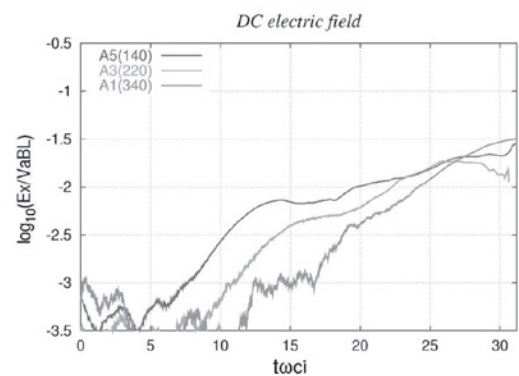
Fig. 2: Time evolutions of DC electric field at the neutral sheet for mass ratios 140, 220 and 340 in varying effective electron mass.
