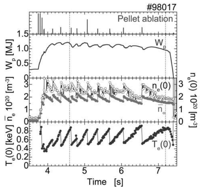
Fig. 1. Time evolution of plasma stored energy W_p , line averaged electron density n_e , central electron density n_e(0) and temperature T_e(0) , together with injection signal of pellet (top).
