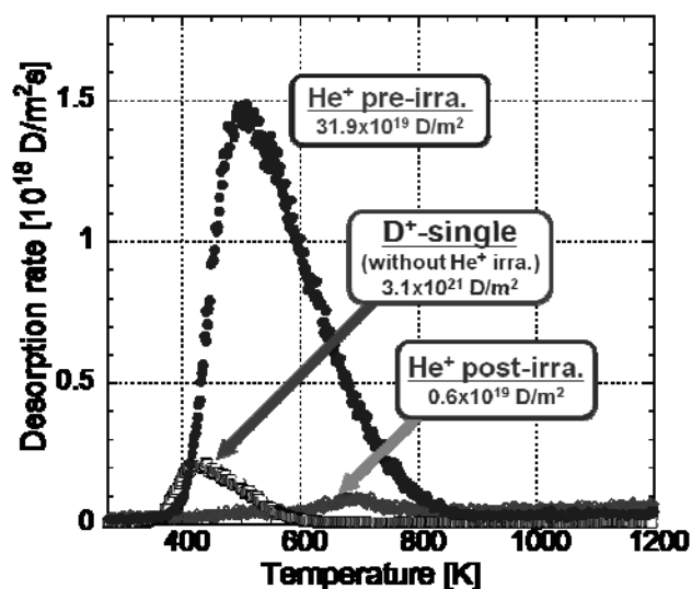
Fig. 2 Thermal desorption spectra of D 2 in W subsequently irradiated with 3 keV-D + of 1 \times 10^{21} D/m 2 before or after the He + irradiation with 3 keV-He + of 10^{21} He/m 2 at R.T.
