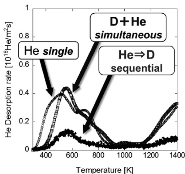
Fig. 2. TDS of He from W irradiated with 3keV-D 2 + ( 1 \times 10^{21} D/m 2 ) and/or 3keV-He + ( 1 \times 10^{21} He/m 2 ).
