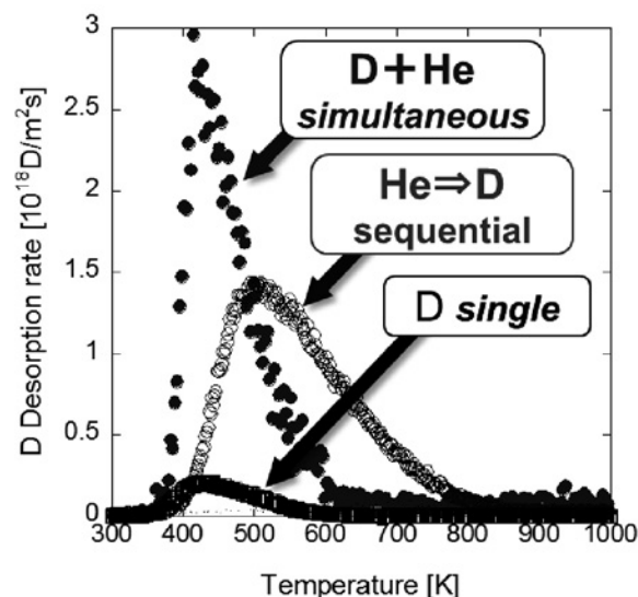
Fig. 1. TDS of D 2 from W irradiated with 3keV-D 2 + ( 1 \times 10^{21} D/m 2 ) and/or 3keV-He + ( 1 \times 10^{21} He/m 2 ).
