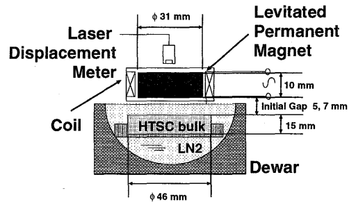
Fig.2: Experimental apparatus
