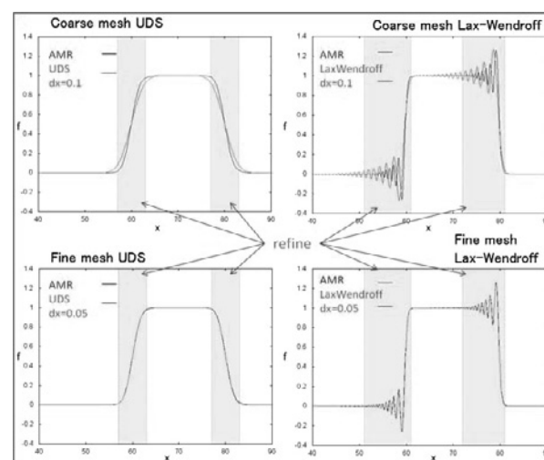
Fig.2 Numerical check of the local refinement by the use of the module.
