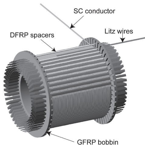
Fig. 1. Structure of conduction-cooled LTS pulse coil.
