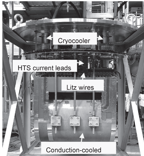
Fig. 2. Cooling and excitation test apparatus for conduction-cooled LTS pulse coil.
