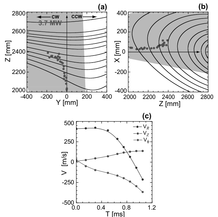
Fig. 2: Trajectory deflection along (a) toroidal plane (b) poloidal plane and (c) ablating pellet speed in radial ( V_R ), vertical ( V_Z ) and toroidal ( V_\phi ) direction in presence of CCW NBI.
