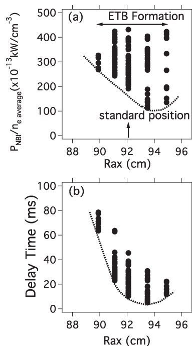
Fig. 1: (a) NBI power values normalized by densities at L-H transition on various magnetic configurations (magnetic axis locations). (b) Delay times from the beam injection. Dotted curves denote the power threshold.
